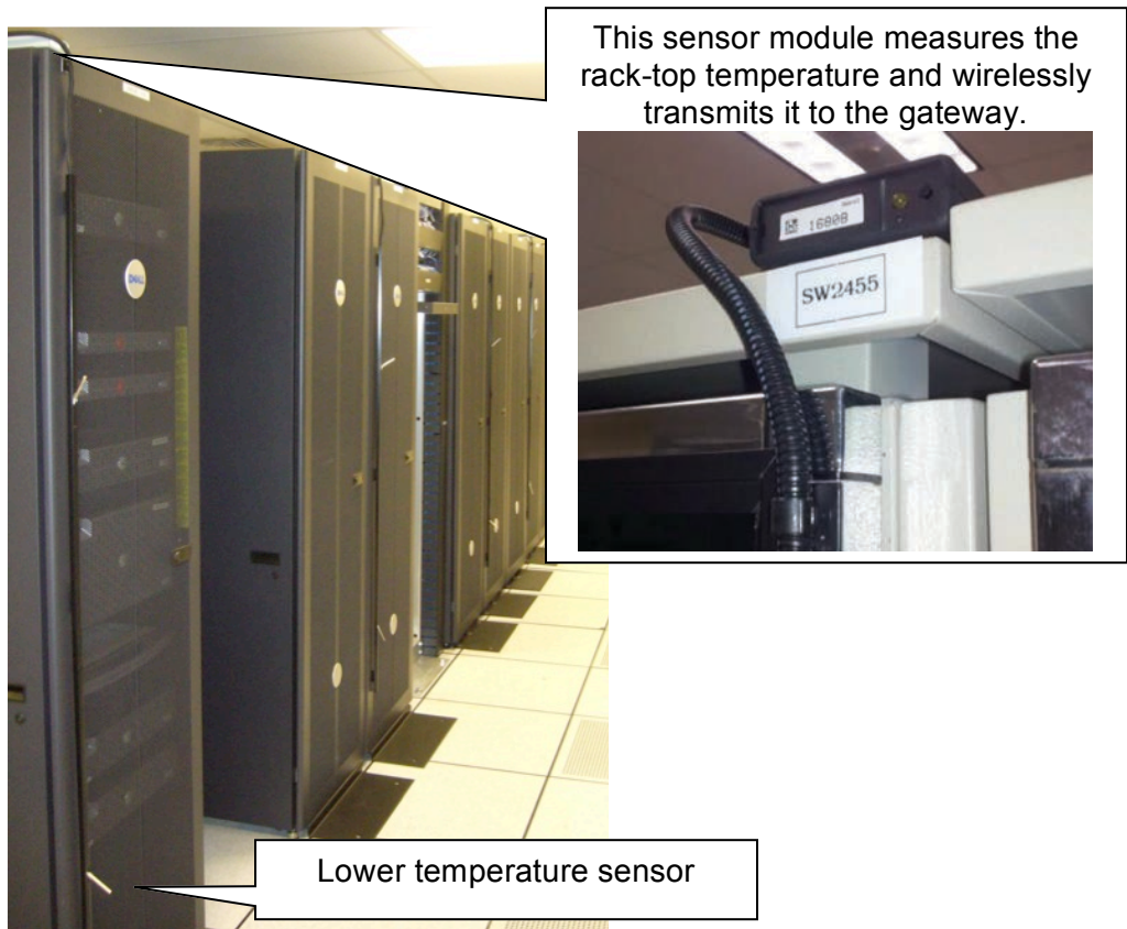
Figure 6: Temperature Sensors
