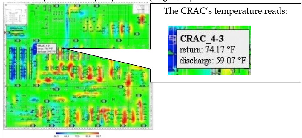
Figure 16: Gold Camp Thermal Map Top of Rack (Aug. 2011)
